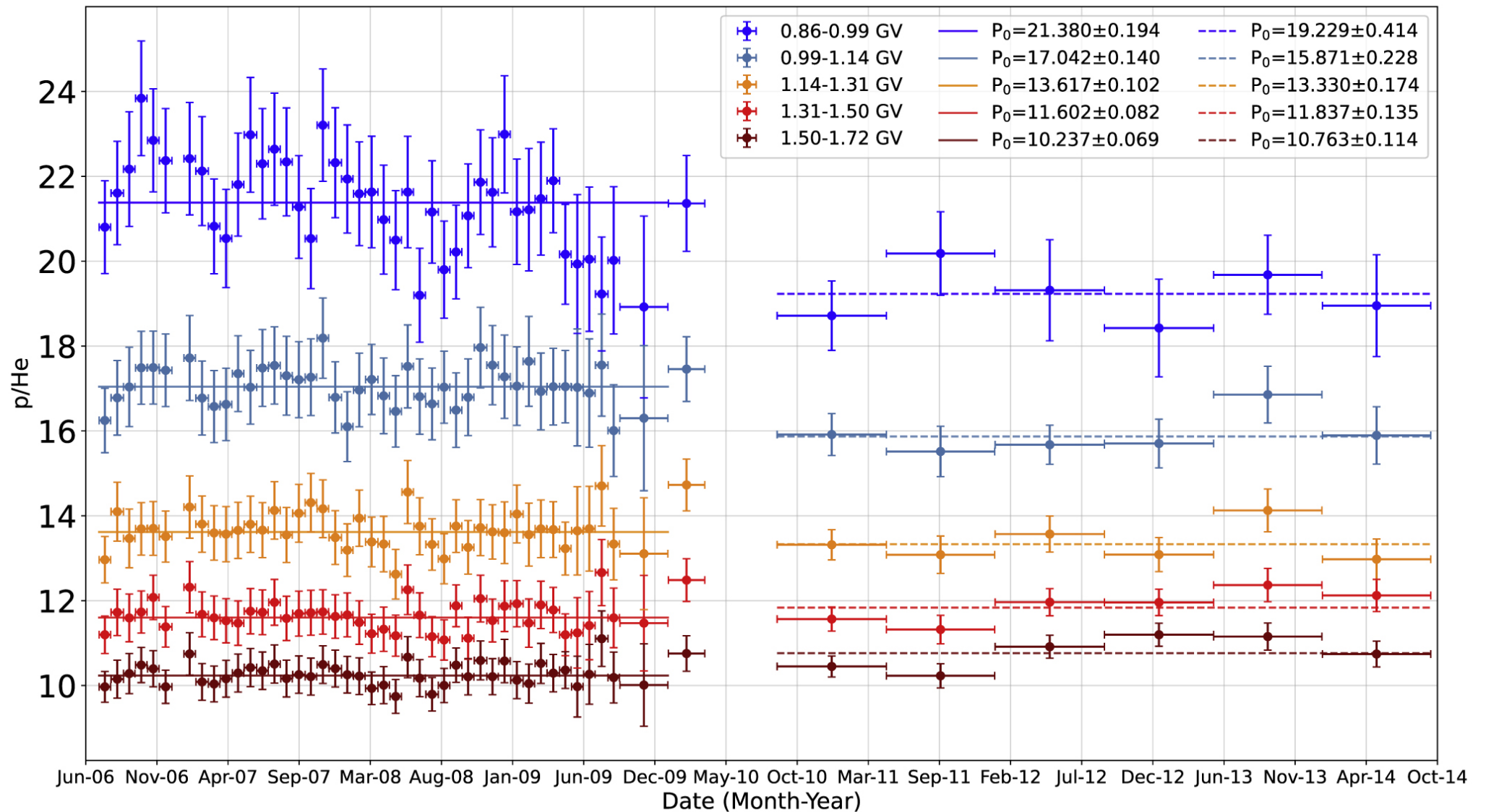
Figure 3. from Helium Fluxes Measured by the PAMELA Experiment from the Minimum to the Maximum Solar Activity for Solar Cycle 24 null 2022 APJL 925 L24 doi:10.3847/2041-8213/ac4787 https://dx.doi.org/10.3847/2041-8213/ac4787 © 2022. The Author(s). Published by the American Astronomical Society.
