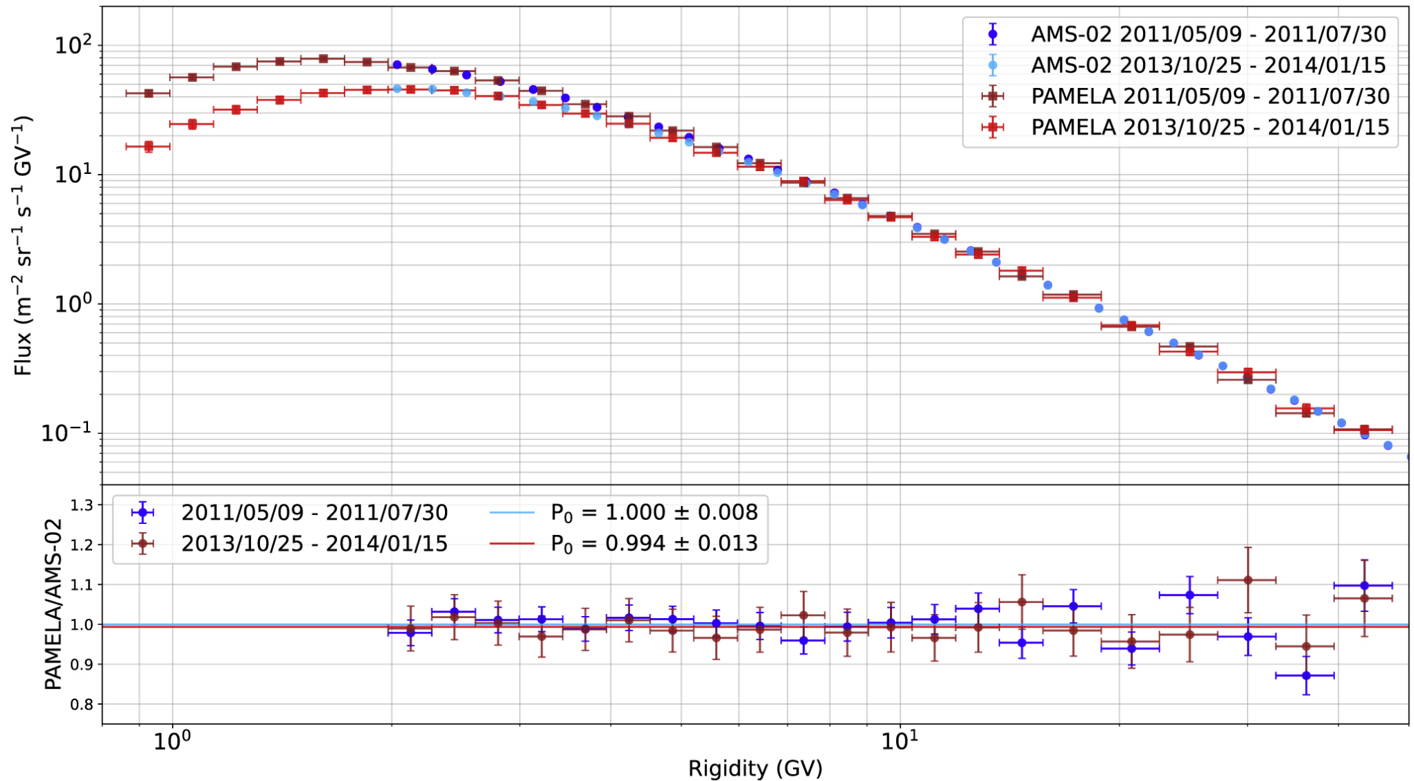
Figure 2. from Helium Fluxes Measured by the PAMELA Experiment from the Minimum to the Maximum Solar Activity for Solar Cycle 24 null 2022 APJL 925 L24 doi:10.3847/2041-8213/ac4787 https://dx.doi.org/10.3847/2041-8213/ac4787 © 2022. The Author(s). Published by the American Astronomical Society.
