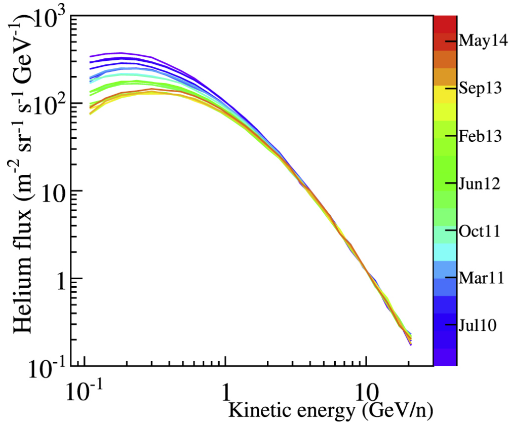
Figure 1. from Helium Fluxes Measured by the PAMELA Experiment from the Minimum to the Maximum Solar Activity for Solar Cycle 24 null 2022 APJL 925 L24 doi:10.3847/2041-8213/ac4787 https://dx.doi.org/10.3847/2041-8213/ac4787 © 2022. The Author(s). Published by the American Astronomical Society.
