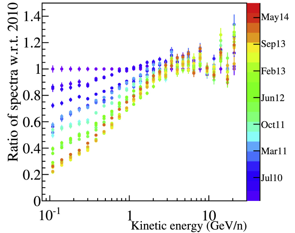
Figure 1. from Helium Fluxes Measured by the PAMELA Experiment from the Minimum to the Maximum Solar Activity for Solar Cycle 24 null 2022 APJL 925 L24 doi:10.3847/2041-8213/ac4787 https://dx.doi.org/10.3847/2041-8213/ac4787 © 2022. The Author(s). Published by the American Astronomical Society.
