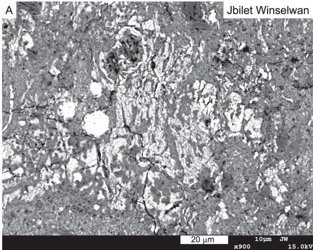
Figure A2. from Wataru Fujiya et al 2022 Astrophys. J. Lett. 924 doi:10.3847/2041-8213/ac448f https://dx.doi.org/10.3847/2041-8213/ac448f © 2022. The Author(s). Published by the American Astronomical Society.
