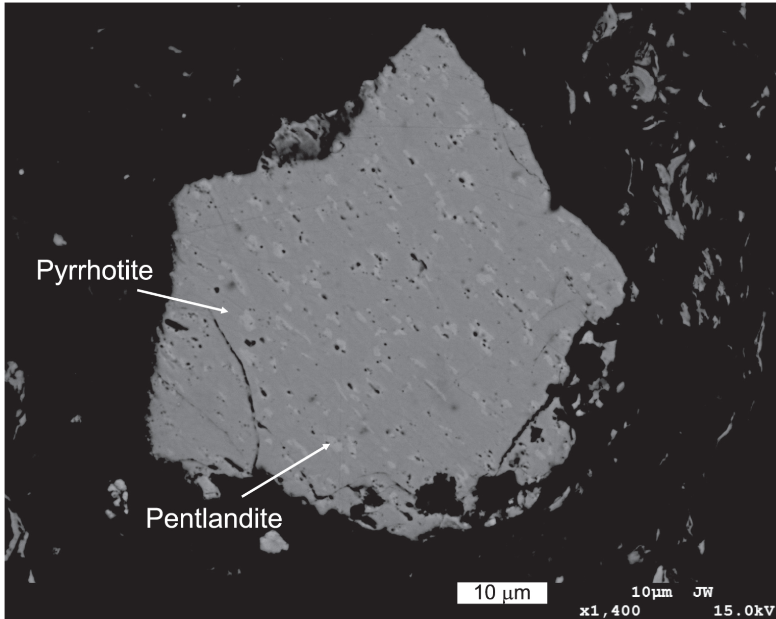
Figure A1. from Wataru Fujiya et al 2022 Astrophys. J. Lett. 924 doi:10.3847/2041-8213/ac448f https://dx.doi.org/10.3847/2041-8213/ac448f © 2022. The Author(s). Published by the American Astronomical Society.
