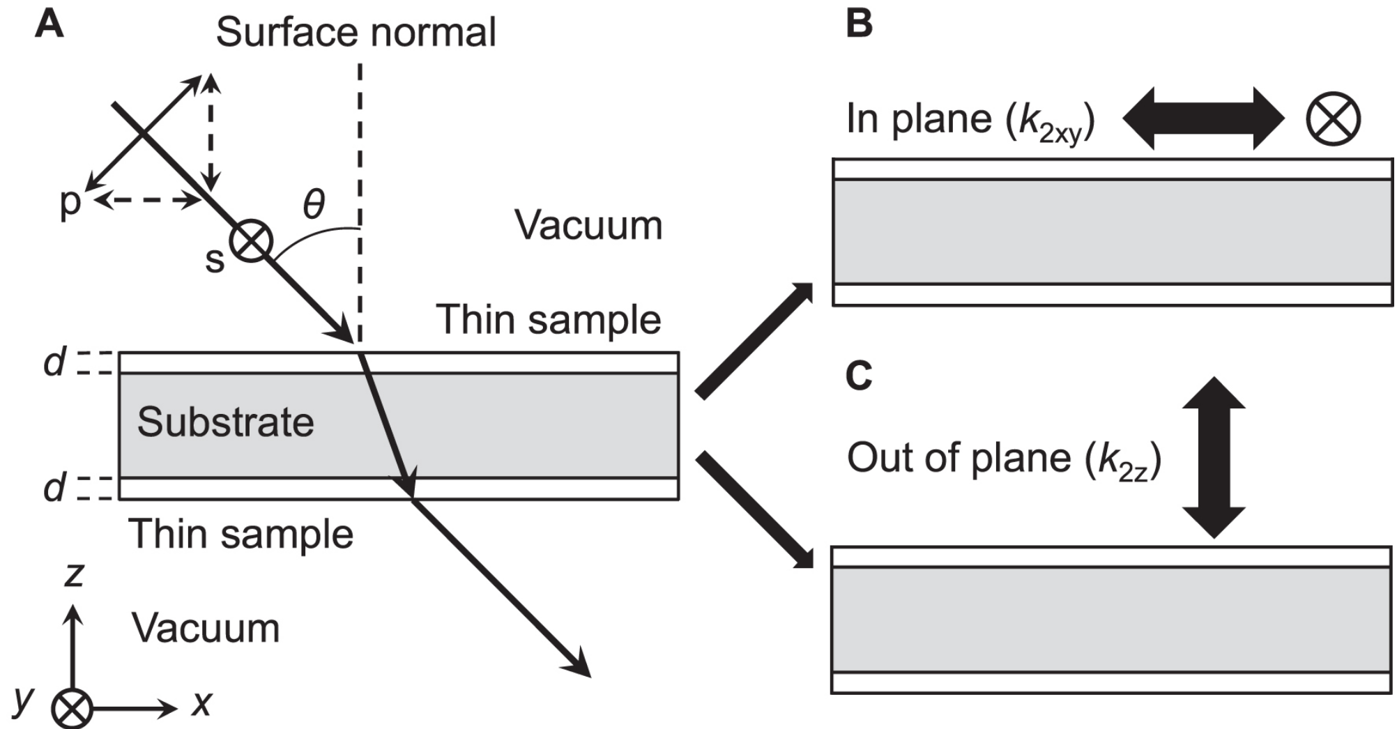
Figure 1. from Absolute Absorption Cross Section and Orientation of Dangling OH Bonds in Water Ice null 2021 APJL 923 L3 doi:10.3847/2041-8213/ac3a0e https://dx.doi.org/10.3847/2041-8213/ac3a0e © 2021. The Author(s). Published by the American Astronomical Society.
