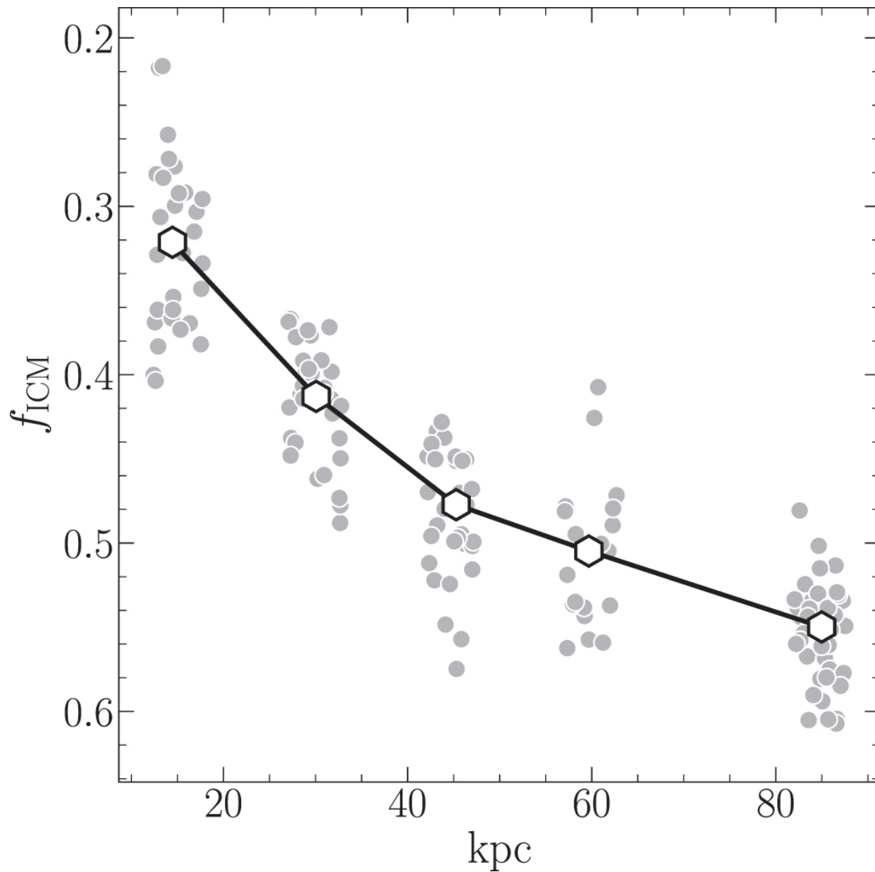
Figure 4. from Andrea Franchetto et al 2021 Astrophys. J. Lett. 922 doi:10.3847/2041-8213/ac3664 https://dx.doi.org/10.3847/2041-8213/ac3664 © 2021. The Author(s). Published by the American Astronomical Society.
