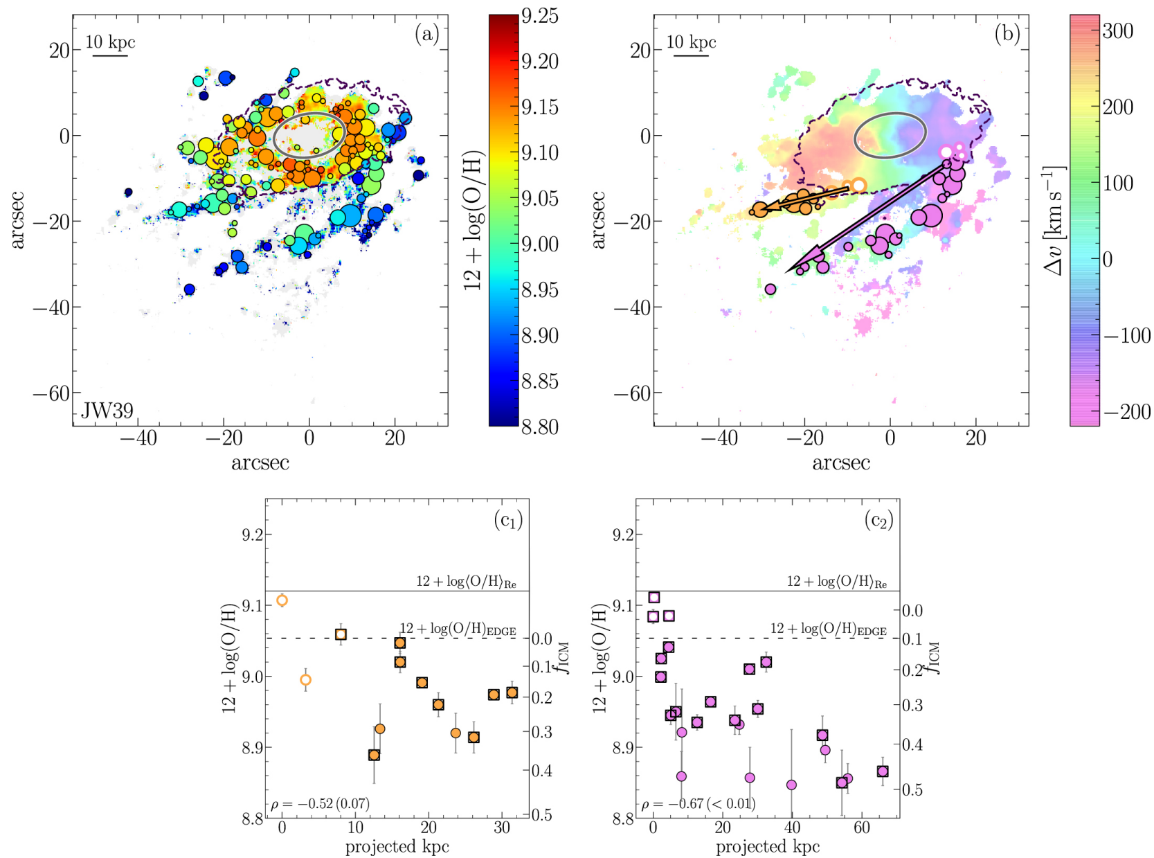
Figure 3. from Andrea Franchetto et al 2021 Astrophys. J. Lett. 922 doi:10.3847/2041-8213/ac3664 https://dx.doi.org/10.3847/2041-8213/ac3664 © 2021. The Author(s). Published by the American Astronomical Society.
