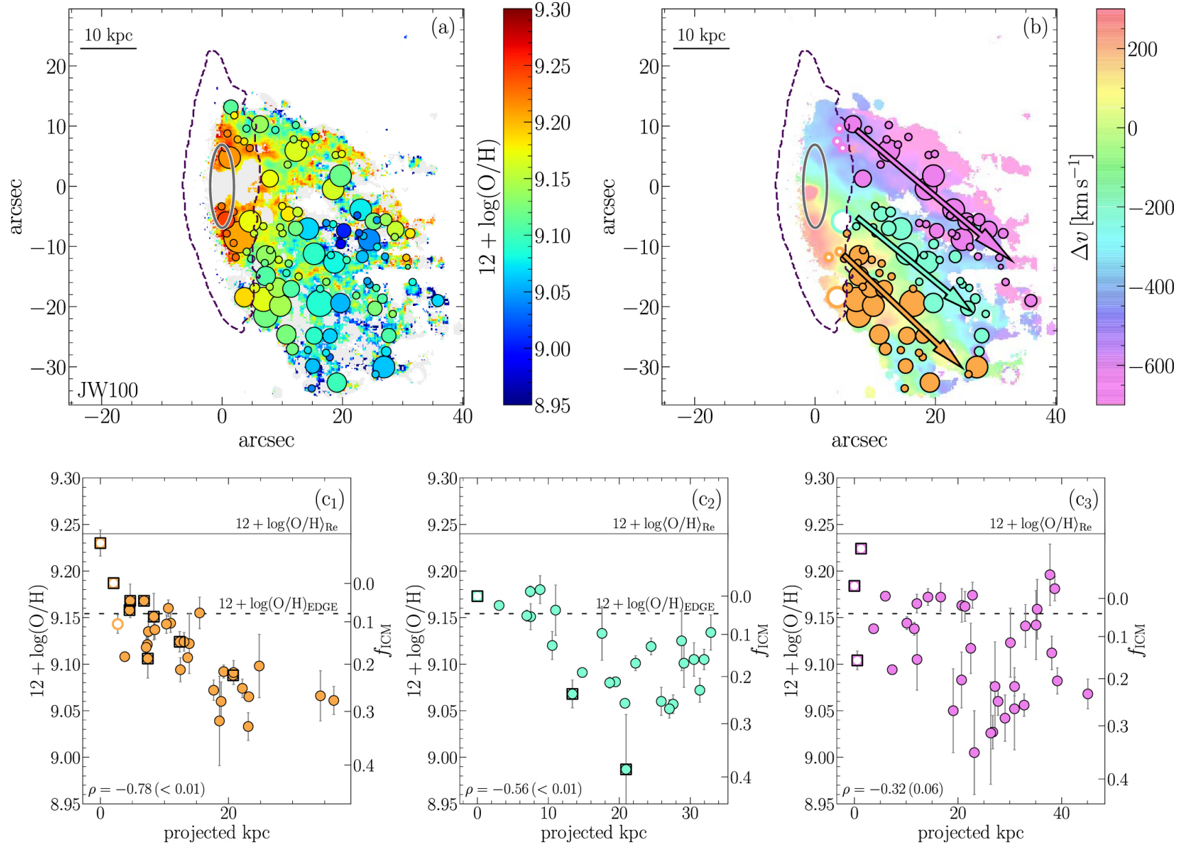
Figure 1. from Andrea Franchetto et al 2021 Astrophys. J. Lett. 922 doi:10.3847/2041-8213/ac3664 https://dx.doi.org/10.3847/2041-8213/ac3664 © 2021. The Author(s). Published by the American Astronomical Society.
