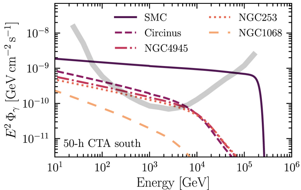
Figure 2. from Antonio Ambrosone et al 2021 Astrophys. J. Lett. 919 doi:10.3847/2041-8213/ac25ff https://dx.doi.org/10.3847/2041-8213/ac25ff © 2021. The American Astronomical Society. All rights reserved.
