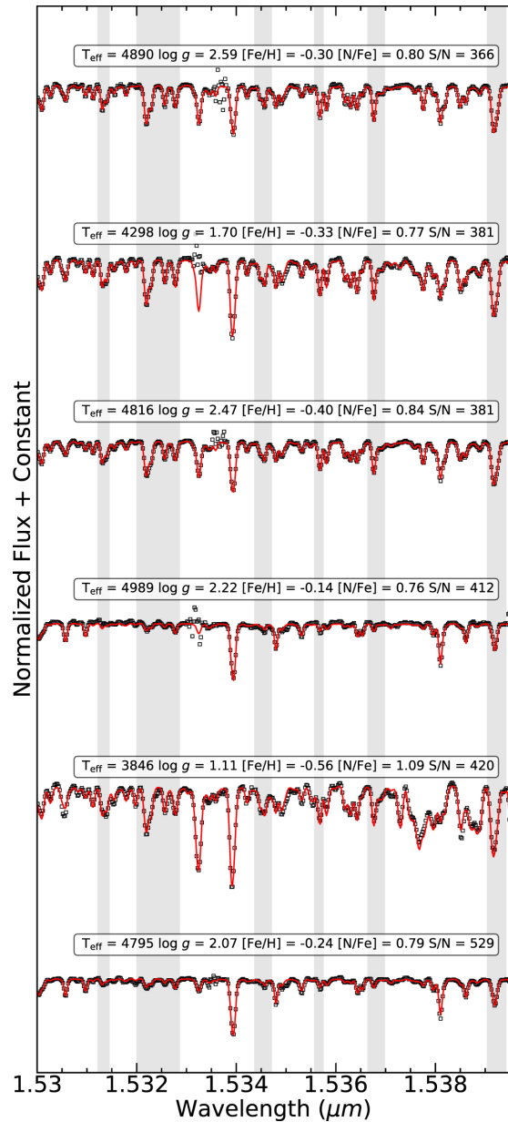
Figure 2. from APOGEE-2 Discovery of a Large Population of Relatively High-metallicity Globular Cluster Debris null 2021 APJL 918 L37 doi:10.3847/2041-8213/ac225b https://dx.doi.org/10.3847/2041-8213/ac225b © 2021. The American Astronomical Society. All rights reserved.
