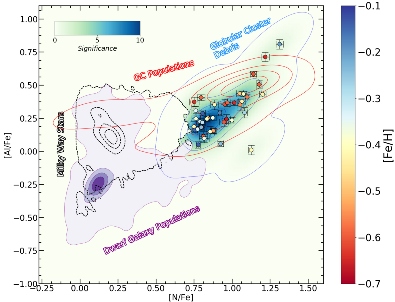
Figure 1. from APOGEE-2 Discovery of a Large Population of Relatively High-metallicity Globular Cluster Debris null 2021 APJL 918 L37 doi:10.3847/2041-8213/ac225b https://dx.doi.org/10.3847/2041-8213/ac225b © 2021. The American Astronomical Society. All rights reserved.
