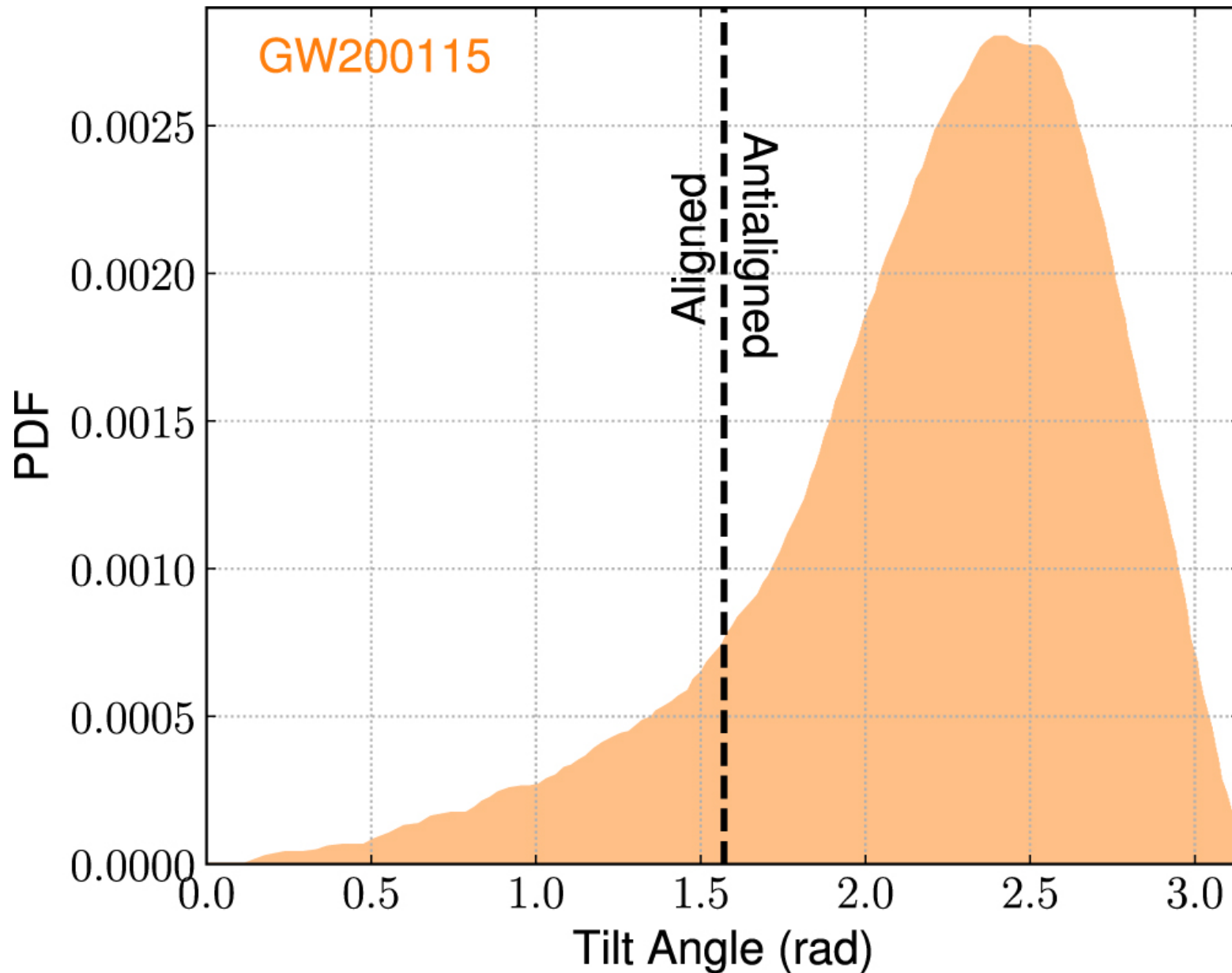
Figure 1. from Impact of Natal Kicks on Merger Rates and Spin–Orbit Misalignments of Black Hole–Neutron Star Mergers null 2021 APJL 918 L38 doi:10.3847/2041-8213/ac225a https://dx.doi.org/10.3847/2041-8213/ac225a © 2021. The American Astronomical Society. All rights reserved.
