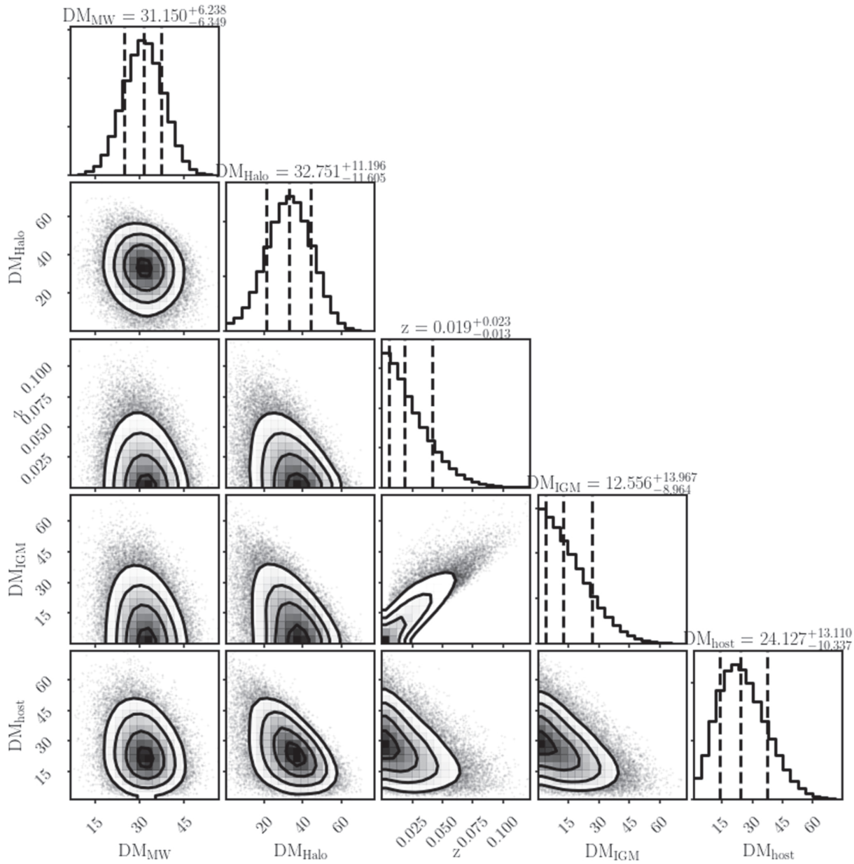
Figure 6. from M. Bhardwaj et al 2021 Astrophys. J. Lett. 919 doi:10.3847/2041-8213/ac223b https://dx.doi.org/10.3847/2041-8213/ac223b © 2021. The American Astronomical Society. All rights reserved.
