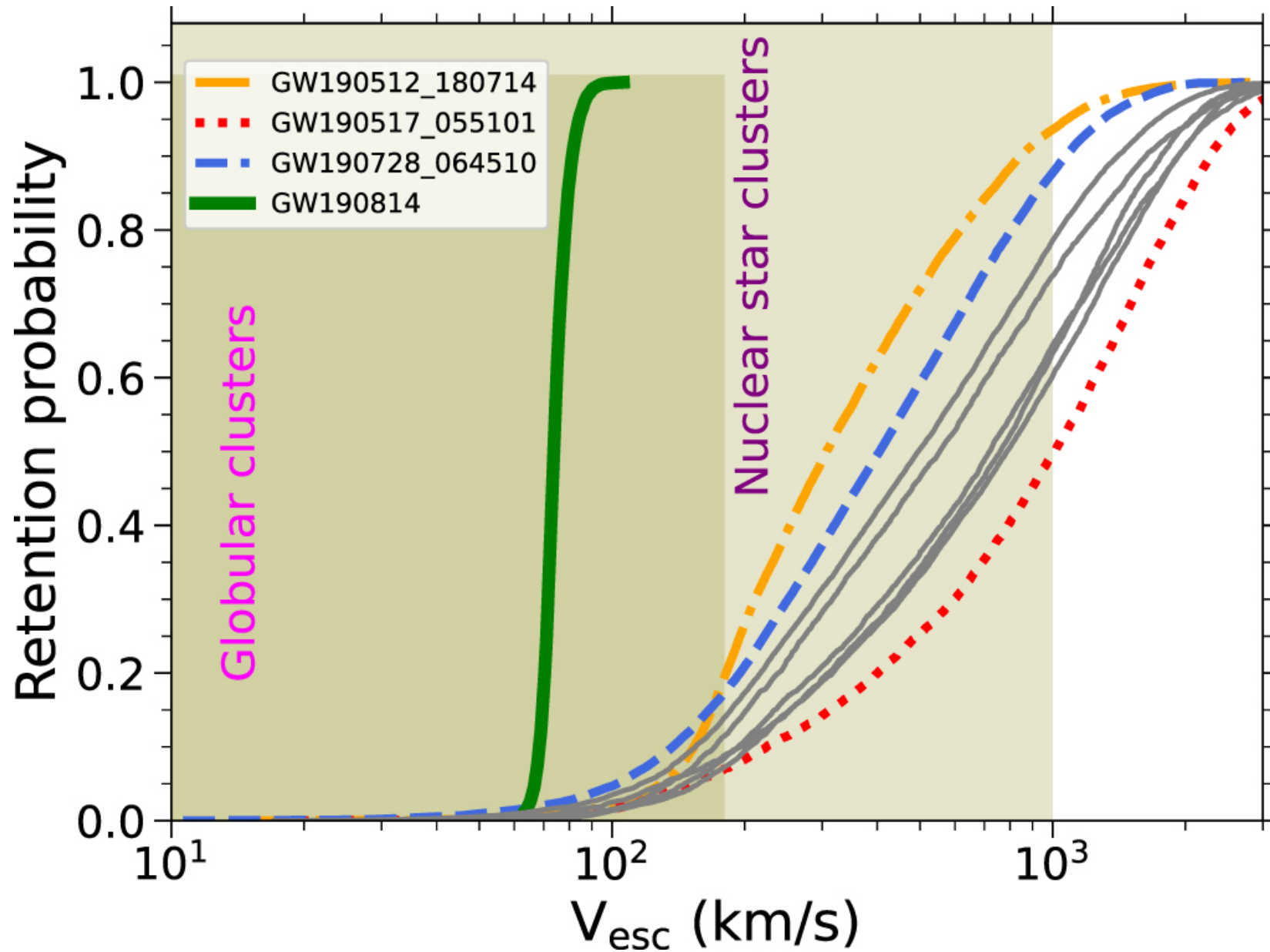
Figure 2. from Remnant Black Hole Kicks and Implications for Hierarchical Mergers null 2021 APJL 918 L31 doi:10.3847/2041-8213/ac20db https://dx.doi.org/10.3847/2041-8213/ac20db © 2021. The American Astronomical Society. All rights reserved.
