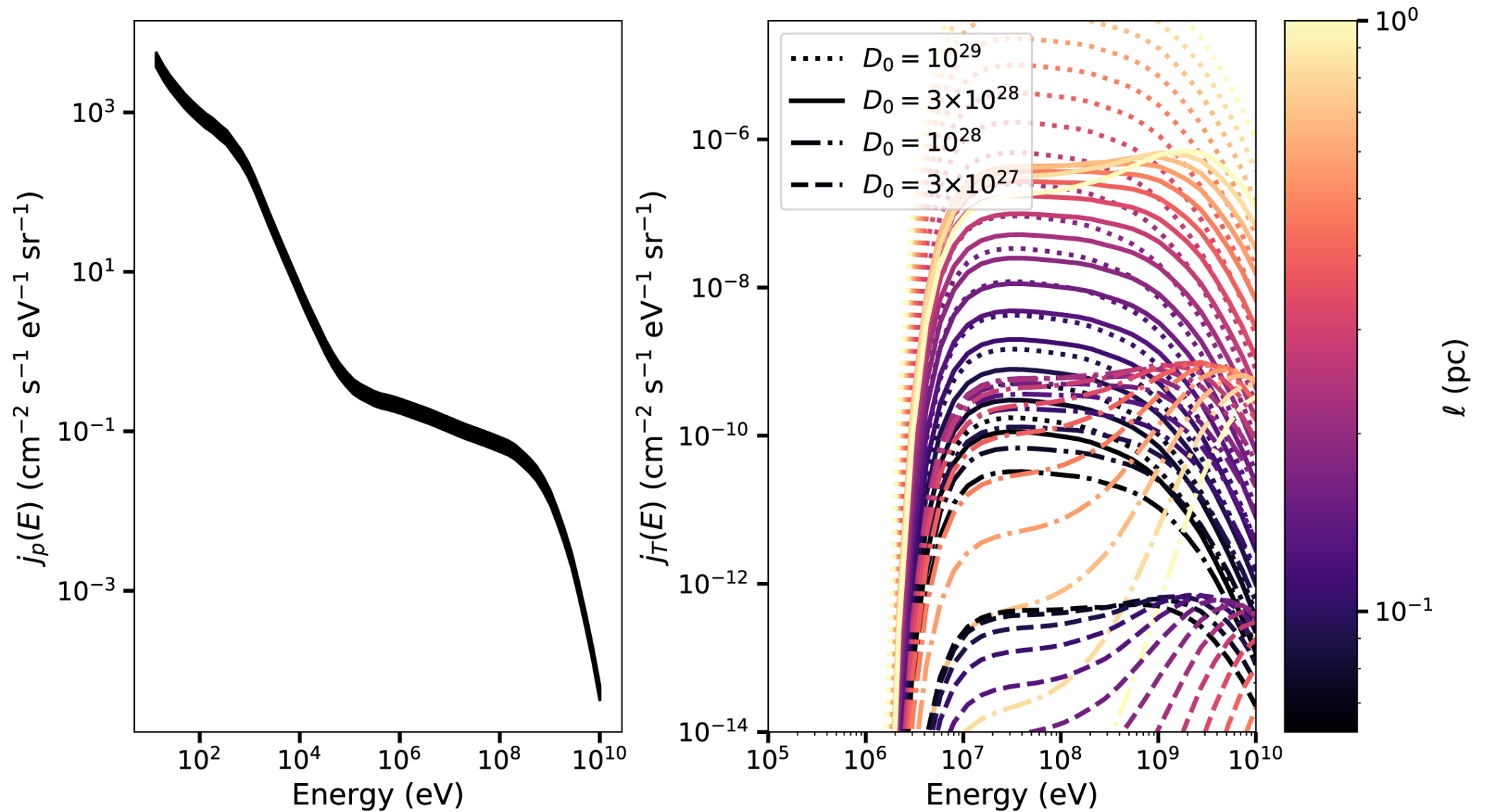
Figure 2. from Cosmic-Ray Acceleration from Turbulence in Molecular Clouds null 2021 APJL 917 L39 doi:10.3847/2041-8213/ac1b2f https://dx.doi.org/10.3847/2041-8213/ac1b2f © 2021. The American Astronomical Society. All rights reserved.
