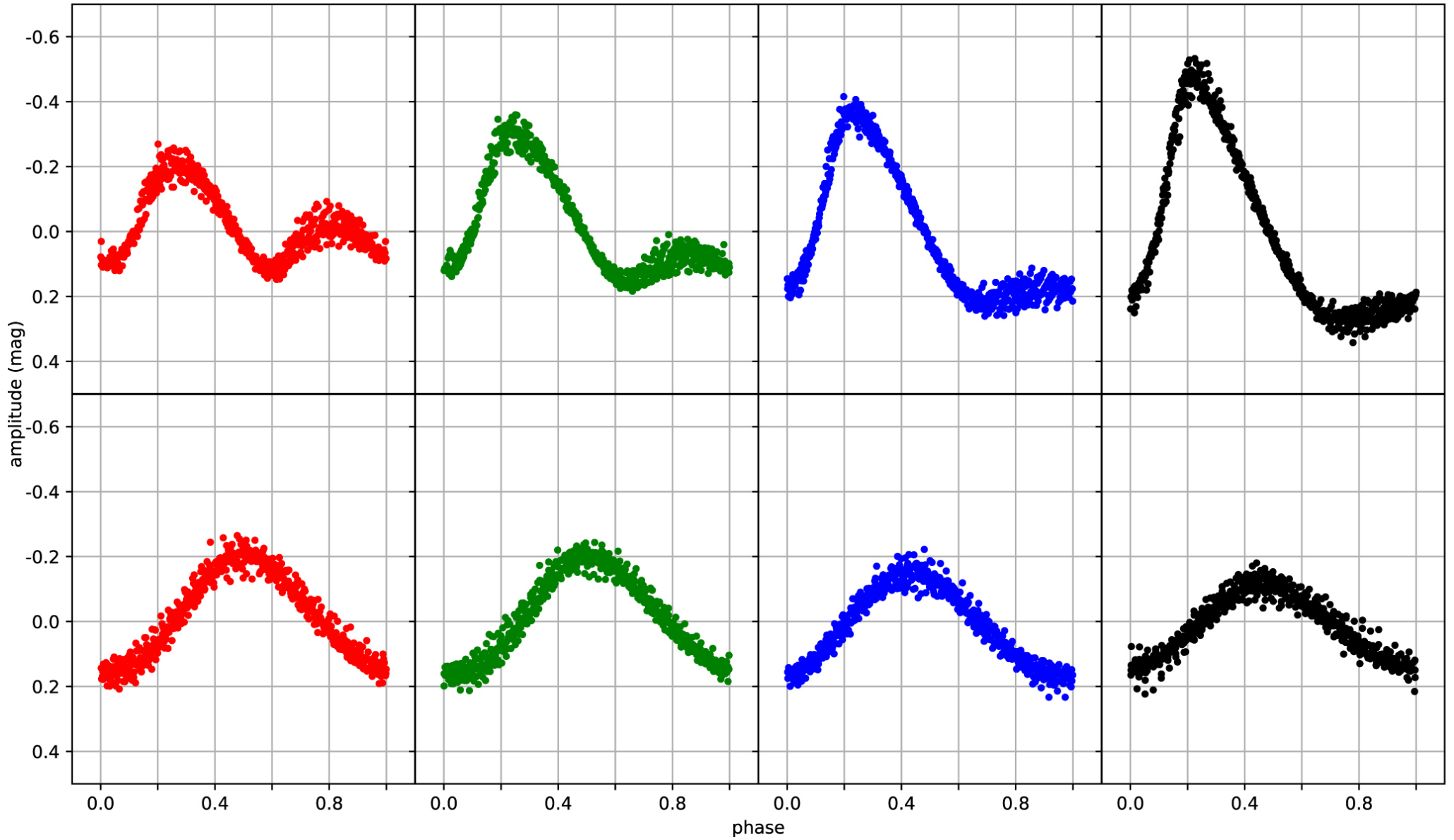
Figure 4. from The Changing Lightcurve of the Double-mode RR Lyrae Variable Star V338 Boo null 2021 APJL 916 L12 doi:10.3847/2041-8213/ac1202 https://dx.doi.org/10.3847/2041-8213/ac1202 © 2021. The American Astronomical Society. All rights reserved.
