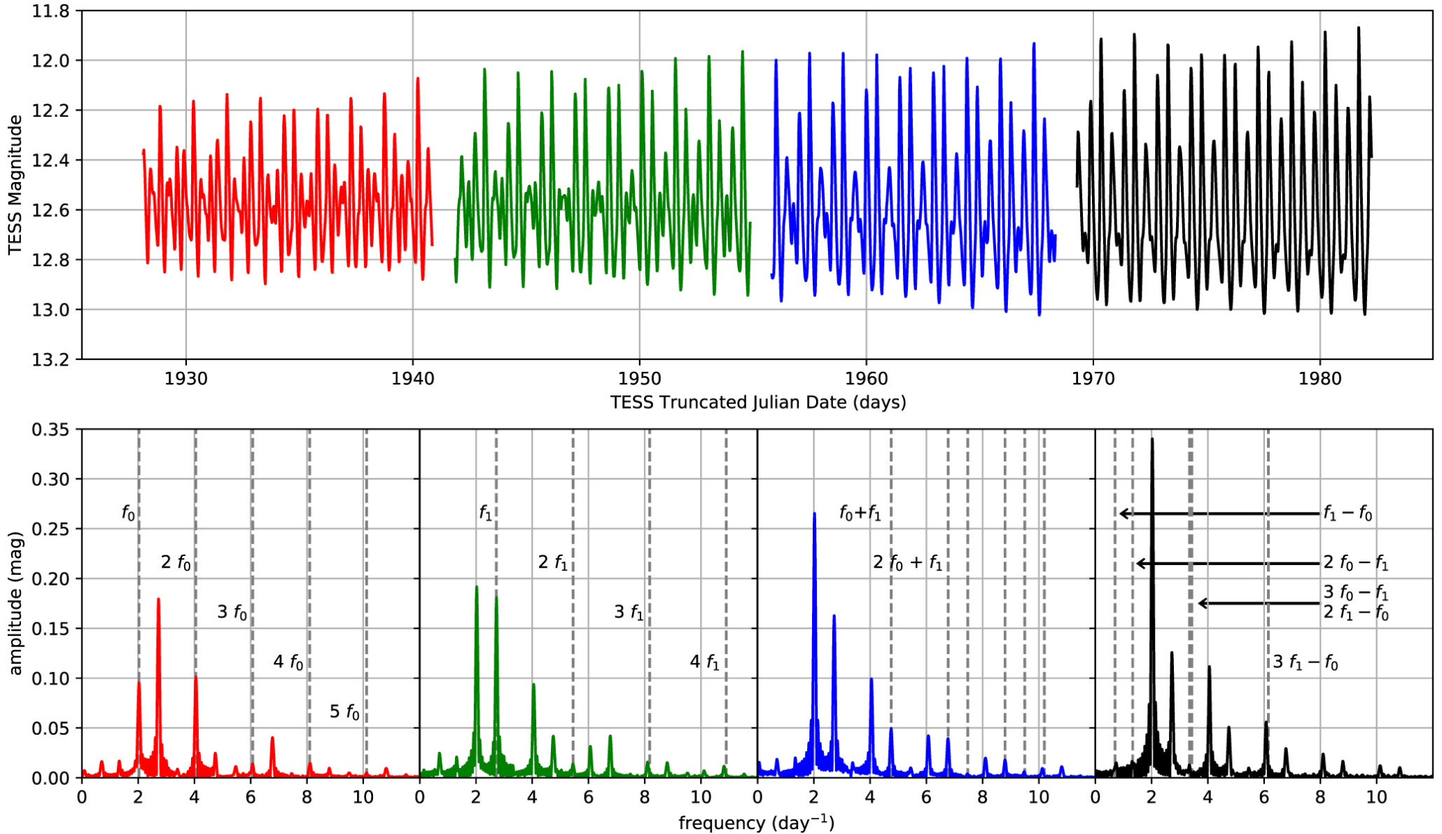
Figure 1. from The Changing Lightcurve of the Double-mode RR Lyrae Variable Star V338 Boo null 2021 APJL 916 L12 doi:10.3847/2041-8213/ac1202 https://dx.doi.org/10.3847/2041-8213/ac1202 © 2021. The American Astronomical Society. All rights reserved.
