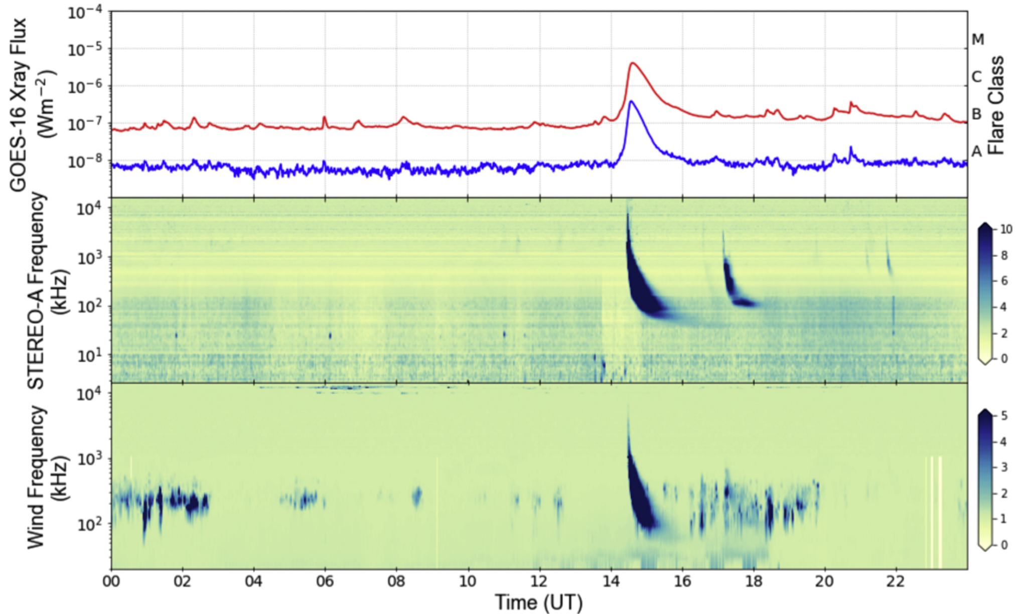
Figure 5. from The Double-bubble Coronal Mass Ejection of the 2020 December 14 Total Solar Eclipse null 2021 APJL 914 L39 doi:10.3847/2041-8213/ac05ca https://dx.doi.org/10.3847/2041-8213/ac05ca © 2021. The American Astronomical Society. All rights reserved.
