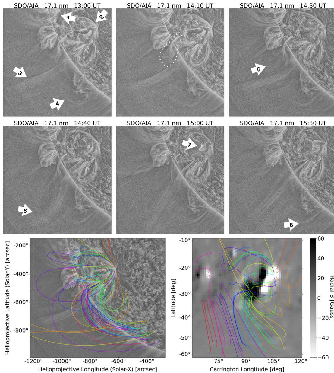
Figure 4. from The Double-bubble Coronal Mass Ejection of the 2020 December 14 Total Solar Eclipse null 2021 APJL 914 L39 doi:10.3847/2041-8213/ac05ca https://dx.doi.org/10.3847/2041-8213/ac05ca
