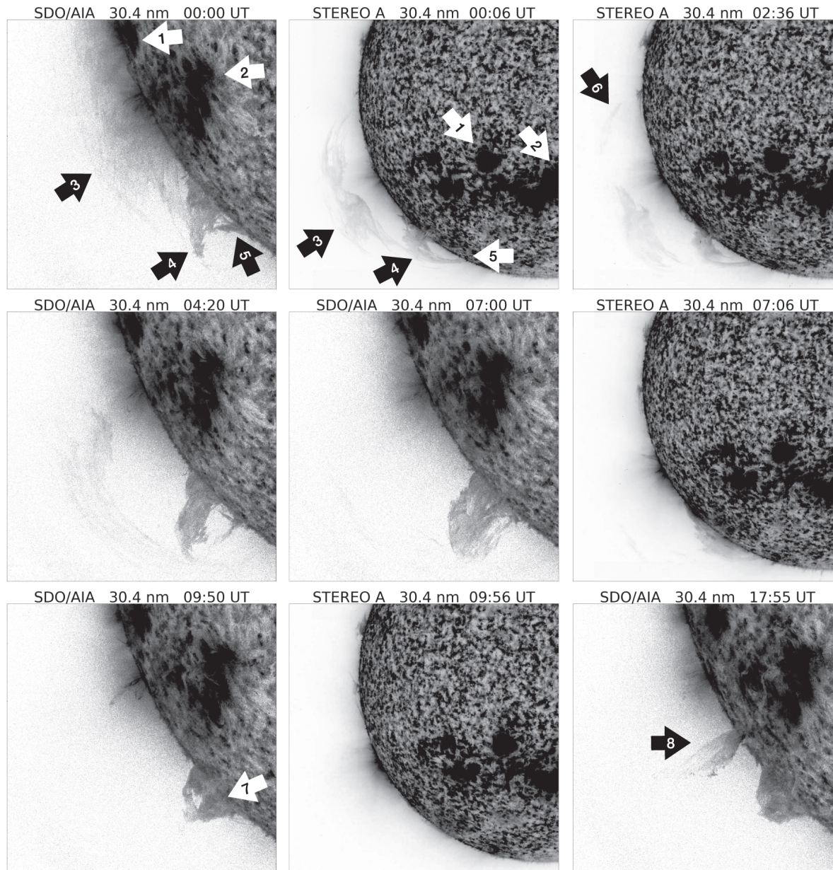
Figure 3. from The Double-bubble Coronal Mass Ejection of the 2020 December 14 Total Solar Eclipse null 2021 APJL 914 L39 doi:10.3847/2041-8213/ac05ca https://dx.doi.org/10.3847/2041-8213/ac05ca © 2021. The American Astronomical Society. All rights reserved.
