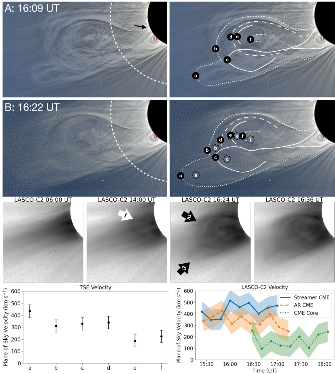
Figure 2. from The Double-bubble Coronal Mass Ejection of the 2020 December 14 Total Solar Eclipse null 2021 APJL 914 L39 doi:10.3847/2041-8213/ac05ca https://dx.doi.org/10.3847/2041-8213/ac05ca © 2021. The American Astronomical Society. All rights reserved.
