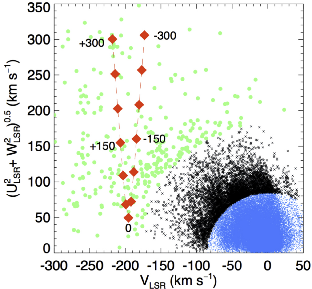
Figure 4. from The Enigmatic Brown Dwarf WISEA J153429.75-104303.3 (a.k.a. “The Accident”) null 2021 APJL 915 L6 doi:10.3847/2041-8213/ac0437 https://dx.doi.org/10.3847/2041-8213/ac0437 © 2021. The American Astronomical Society. All rights reserved.
