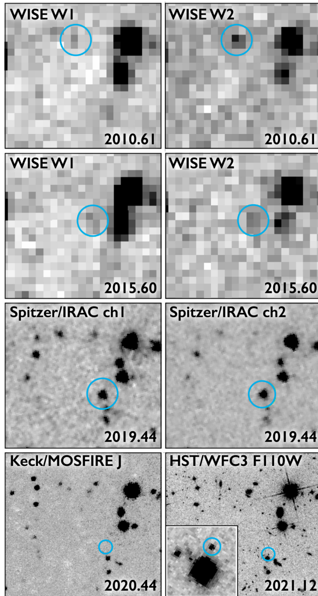
Figure 1. from The Enigmatic Brown Dwarf WISEA J153429.75-104303.3 (a.k.a. “The Accident”) null 2021 APJL 915 L6 doi:10.3847/2041-8213/ac0437 https://dx.doi.org/10.3847/2041-8213/ac0437 © 2021. The American Astronomical Society. All rights reserved.
