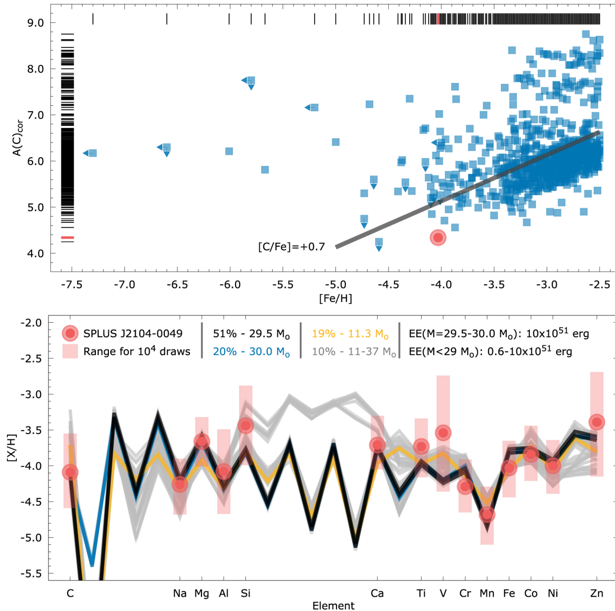
Figure 3. from SPLUS J210428.01004934.2: An Ultra Metal-poor Star Identified from Narrowband Photometry null 2021 APJL 912 L32 doi:10.3847/2041-8213/abf93d https://dx.doi.org/10.3847/2041-8213/abf93d © 2021. The American Astronomical Society. All rights reserved.
