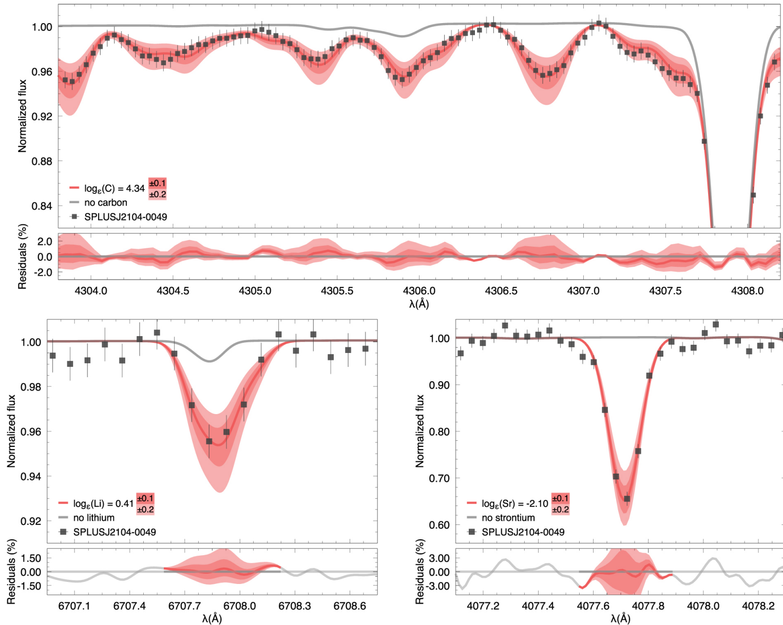
Figure 2. from SPLUS J210428.01004934.2: An Ultra Metal-poor Star Identified from Narrowband Photometry null 2021 APJL 912 L32 doi:10.3847/2041-8213/abf93d https://dx.doi.org/10.3847/2041-8213/abf93d © 2021. The American Astronomical Society. All rights reserved.
