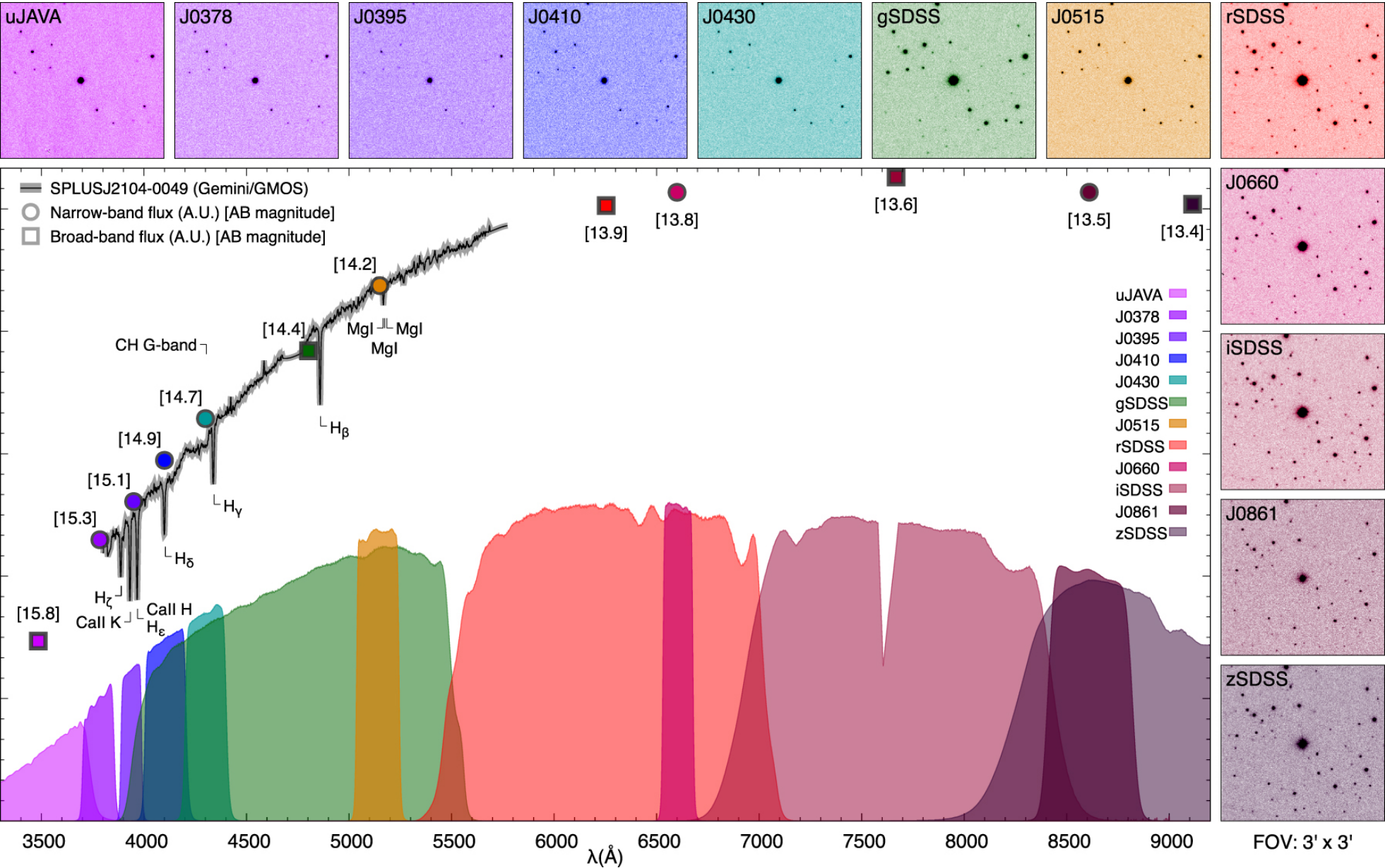
Figure 1. from SPLUS J210428.01004934.2: An Ultra Metal-poor Star Identified from Narrowband Photometry null 2021 APJL 912 L32 doi:10.3847/2041-8213/abf93d https://dx.doi.org/10.3847/2041-8213/abf93d © 2021. The American Astronomical Society. All rights reserved.
