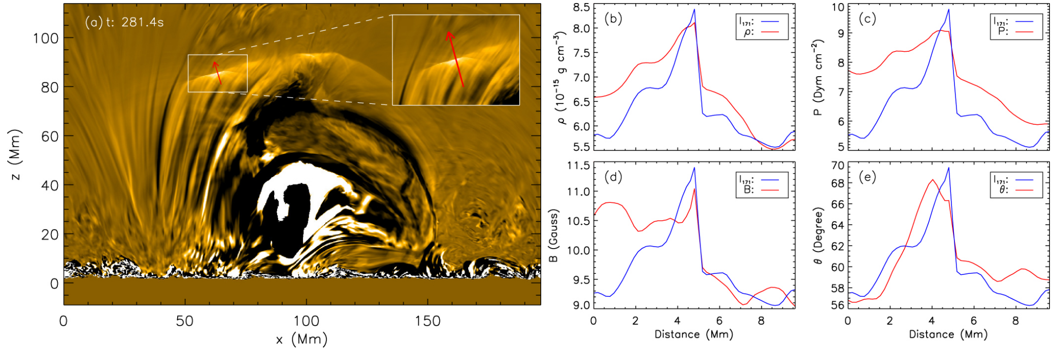
Figure 5. from Exploring the Nature of EUV Waves in a Radiative Magnetohydrodynamic Simulation null 2021 APJL 911 L8 doi:10.3847/2041-8213/abefe6 https://dx.doi.org/10.3847/2041-8213/abefe6 © 2021. The American Astronomical Society. All rights reserved.
