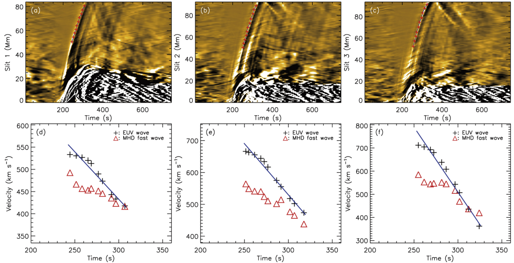
Figure 4. from Exploring the Nature of EUV Waves in a Radiative Magnetohydrodynamic Simulation null 2021 APJL 911 L8 doi:10.3847/2041-8213/abefe6 https://dx.doi.org/10.3847/2041-8213/abefe6 © 2021. The American Astronomical Society. All rights reserved.
