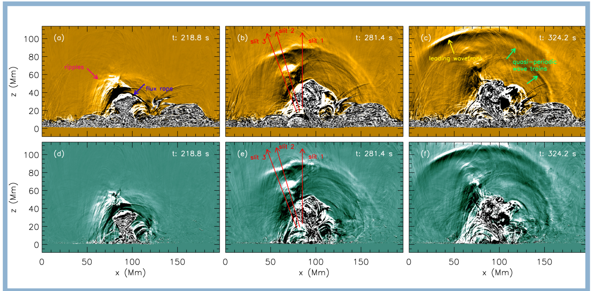
Figure 2. from Exploring the Nature of EUV Waves in a Radiative Magnetohydrodynamic Simulation null 2021 APJL 911 L8 doi:10.3847/2041-8213/abefe6 https://dx.doi.org/10.3847/2041-8213/abefe6 © 2021. The American Astronomical Society. All rights reserved.
