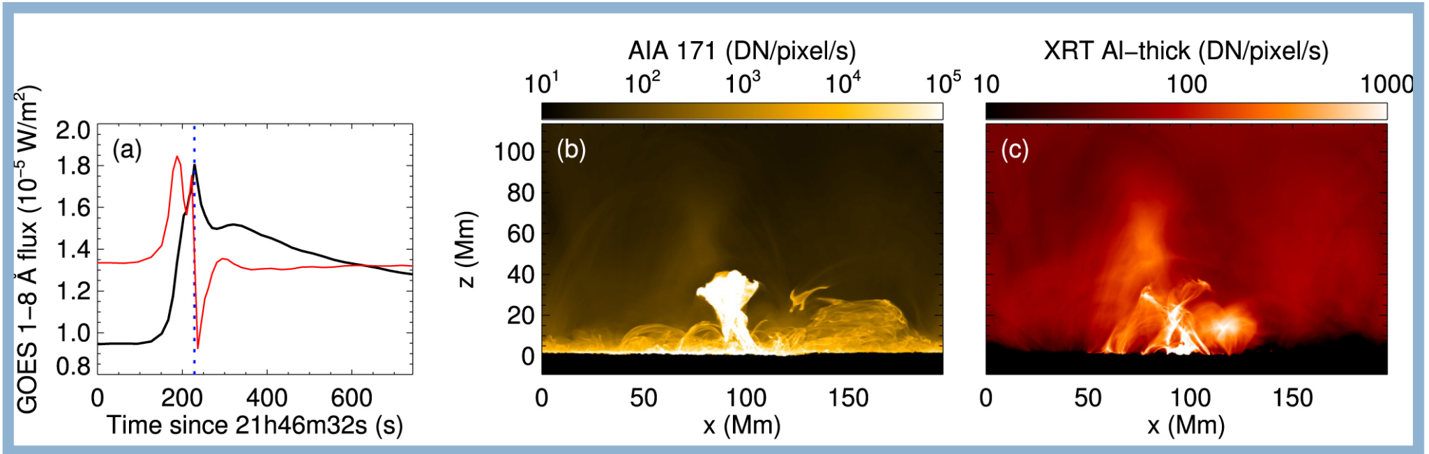
Figure 1. from Exploring the Nature of EUV Waves in a Radiative Magnetohydrodynamic Simulation null 2021 APJL 911 L8 doi:10.3847/2041-8213/abefe6 https://dx.doi.org/10.3847/2041-8213/abefe6 © 2021. The American Astronomical Society. All rights reserved.
