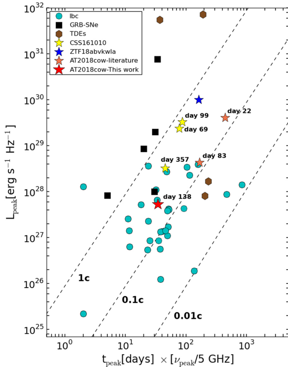
Figure 3. from uGMRT Observations of a Fast and Blue Optical Transient—AT 2018cow null 2021 APJL 912 L9 doi:10.3847/2041-8213/abed55 https://dx.doi.org/10.3847/2041-8213/abed55
