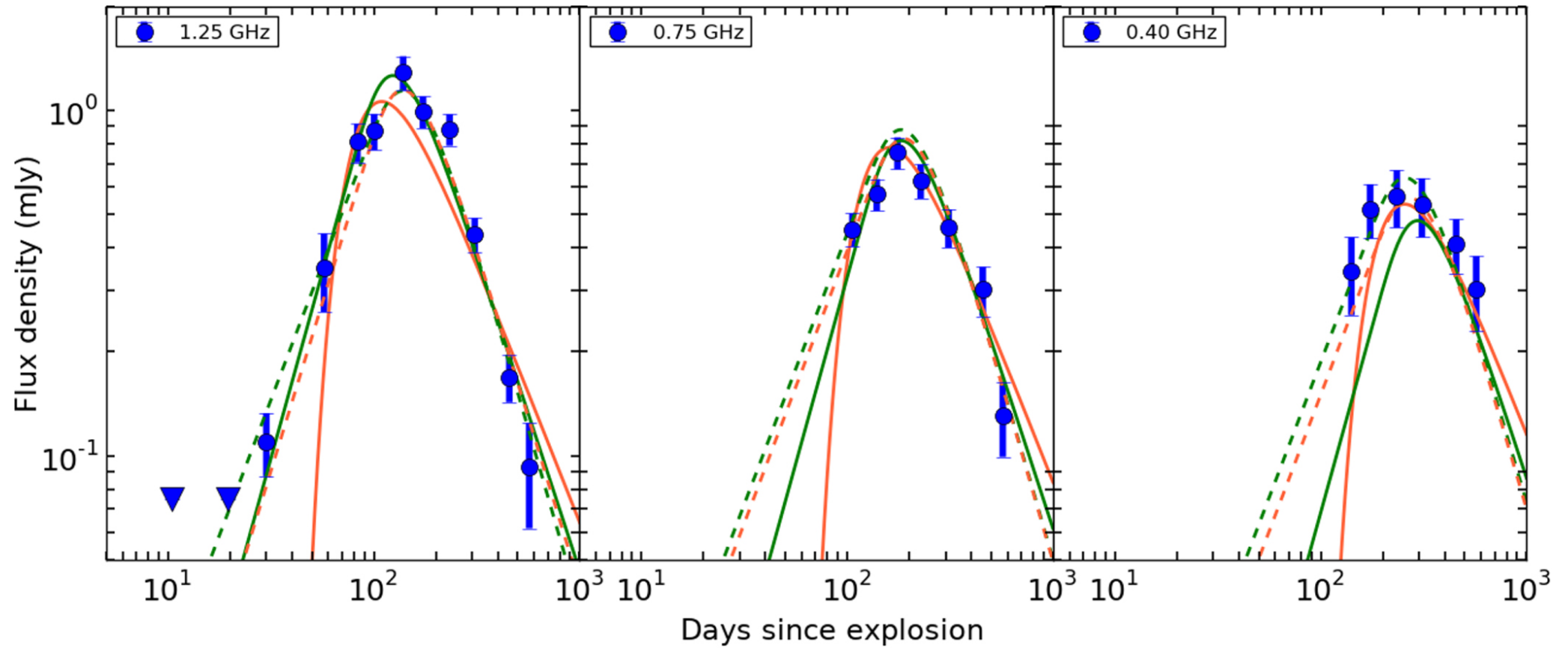
Figure 2. from uGMRT Observations of a Fast and Blue Optical Transient—AT 2018cow null 2021 APJL 912 L9 doi:10.3847/2041-8213/abed55 https://dx.doi.org/10.3847/2041-8213/abed55 © 2021. The American Astronomical Society. All rights reserved.
