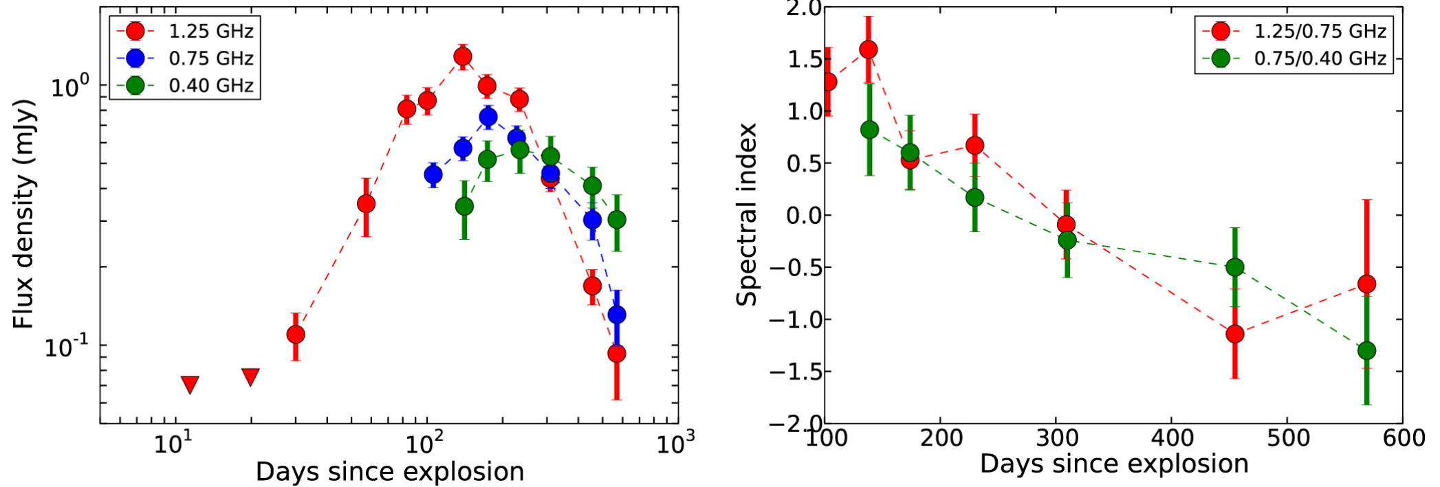
Figure 1. from uGMRT Observations of a Fast and Blue Optical Transient—AT 2018cow null 2021 APJL 912 L9 doi:10.3847/2041-8213/abed55 https://dx.doi.org/10.3847/2041-8213/abed55 © 2021. The American Astronomical Society. All rights reserved.
