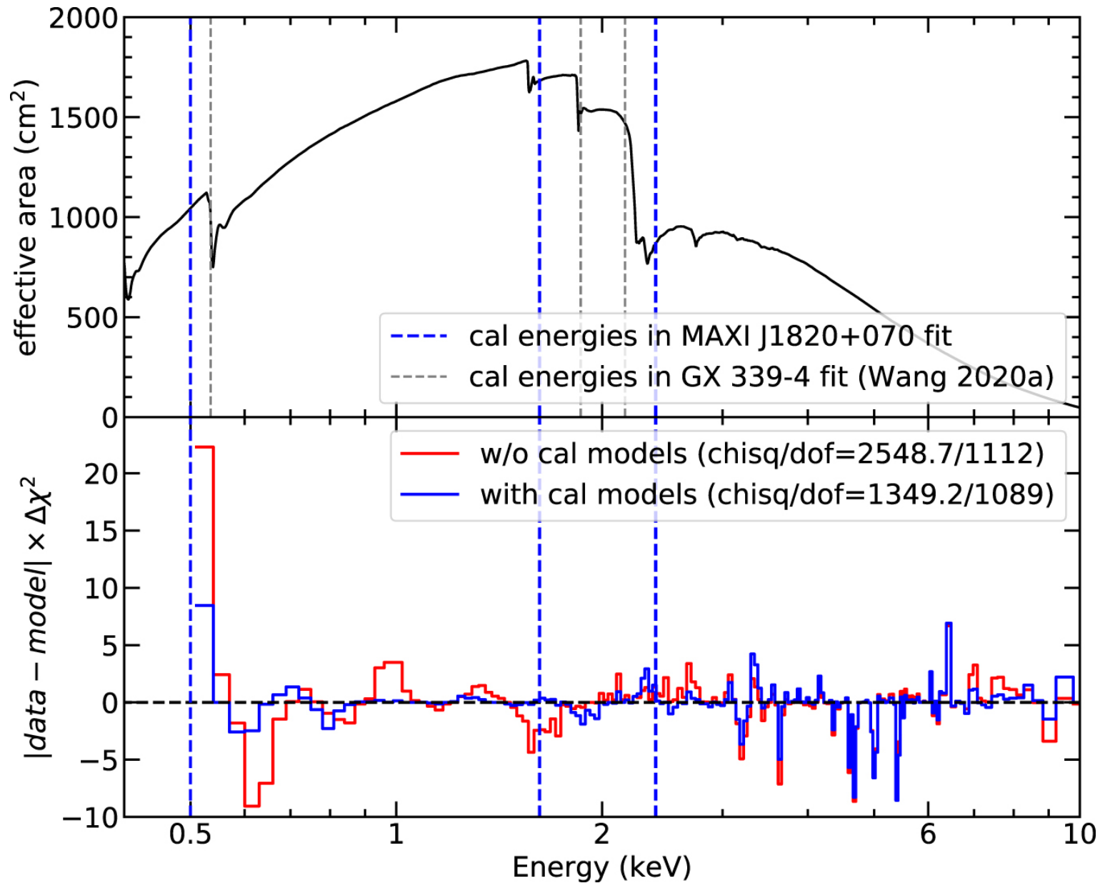
Figure B1. from Disk, Corona, Jet Connection in the Intermediate State of MAXI J1820+070 Revealed by NICER Spectral-timing Analysis null 2021 APJL 910 L3 doi:10.3847/2041-8213/abec79 https://dx.doi.org/10.3847/2041-8213/abec79 © 2021. The American Astronomical Society. All rights reserved.
