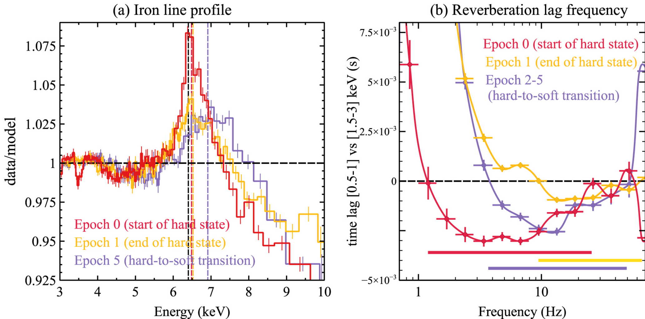
Figure 2. from Disk, Corona, Jet Connection in the Intermediate State of MAXI J1820+070 Revealed by NICER Spectral-timing Analysis null 2021 APJL 910 L3 doi:10.3847/2041-8213/abec79 https://dx.doi.org/10.3847/2041-8213/abec79 © 2021. The American Astronomical Society. All rights reserved.
