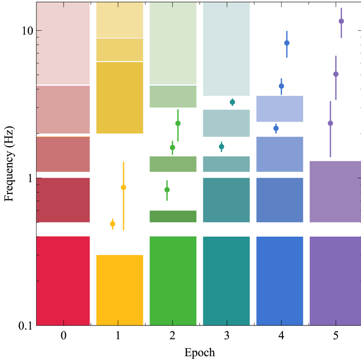
Figure C2. from Disk, Corona, Jet Connection in the Intermediate State of MAXI J1820+070 Revealed by NICER Spectral-timing Analysis null 2021 APJL 910 L3 doi:10.3847/2041-8213/abec79 https://dx.doi.org/10.3847/2041-8213/abec79 © 2021. The American Astronomical Society. All rights reserved.
