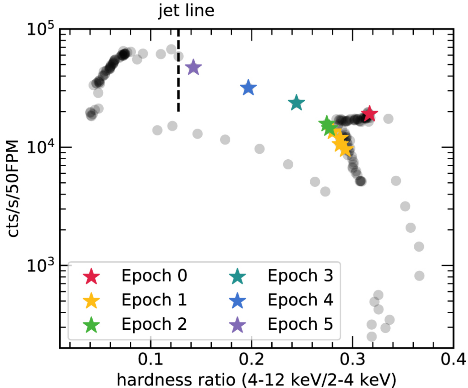
Figure 1. from Disk, Corona, Jet Connection in the Intermediate State of MAXI J1820+070 Revealed by NICER Spectral-timing Analysis null 2021 APJL 910 L3 doi:10.3847/2041-8213/abec79 https://dx.doi.org/10.3847/2041-8213/abec79 © 2021. The American Astronomical Society. All rights reserved.
