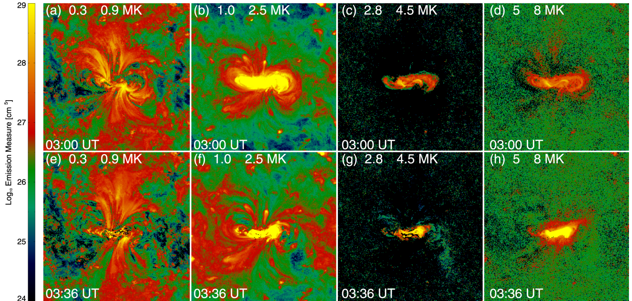
Figure 5. from Diagnosing a Solar Flaring Core with Bidirectional Quasi-periodic Fast Propagating Magnetoacoustic Waves null 2021 APJL 908 L37 doi:10.3847/2041-8213/abdfce https://dx.doi.org/10.3847/2041-8213/abdfce
