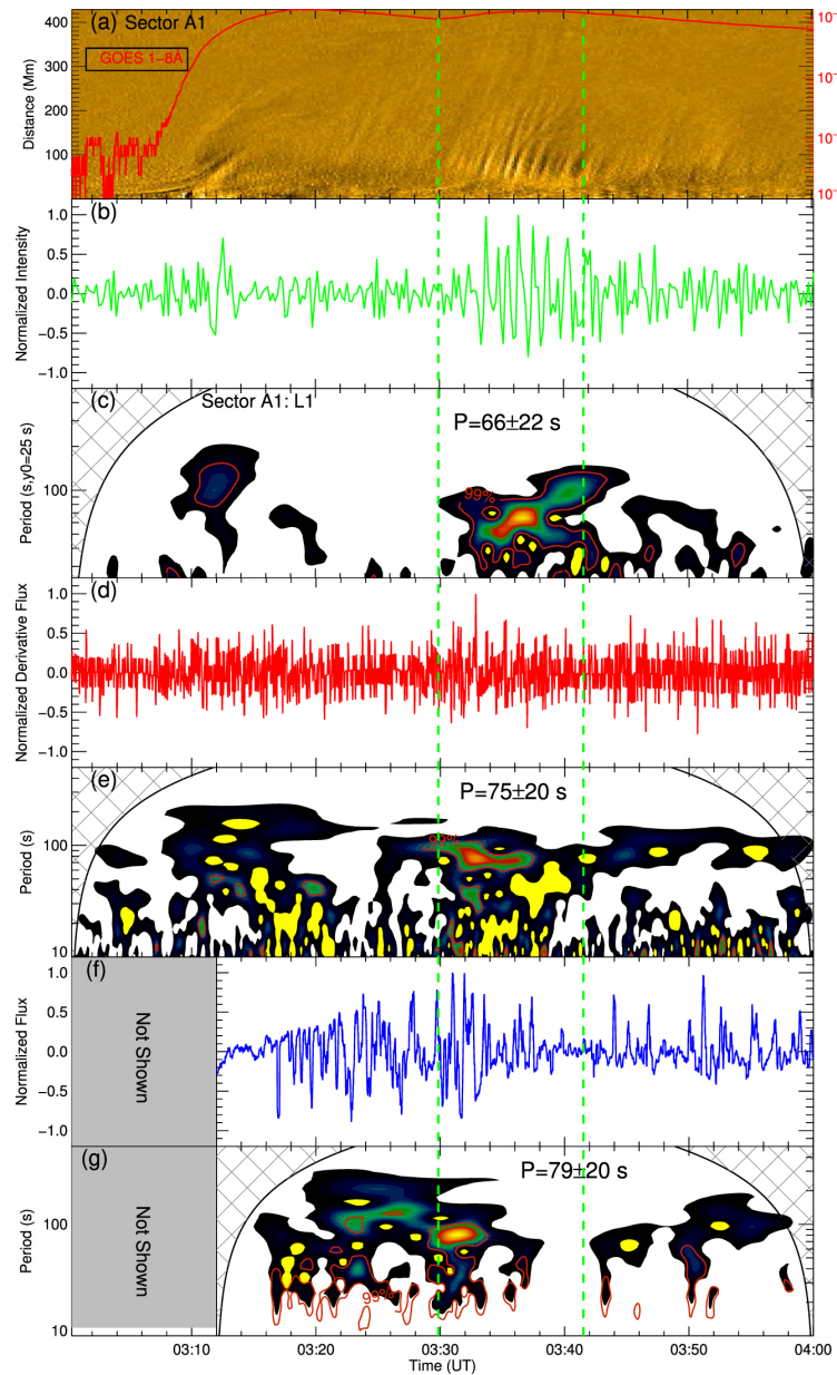
Figure 3. from Diagnosing a Solar Flaring Core with Bidirectional Quasi-periodic Fast Propagating Magnetoacoustic Waves null 2021 APJL 908 L37 doi:10.3847/2041-8213/abdfce https://dx.doi.org/10.3847/2041-8213/abdfce
