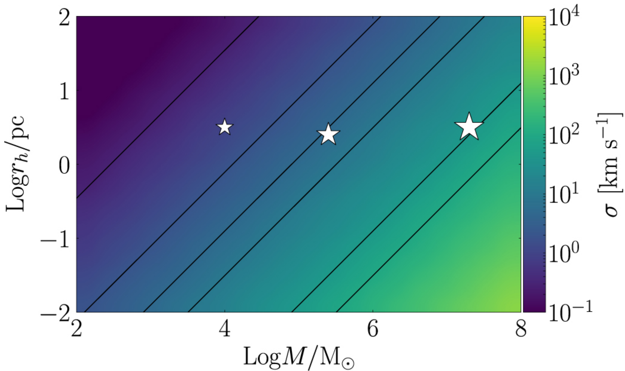
Figure 8. from Dynamical Formation of the GW190814 Merger null 2021 APJL 908 L38 doi:10.3847/2041-8213/abdfcd https://dx.doi.org/10.3847/2041-8213/abdfcd © 2021. The American Astronomical Society. All rights reserved.
