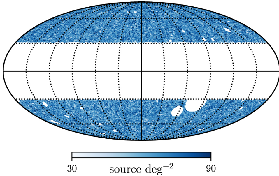
Figure 1. from A Test of the Cosmological Principle with Quasars null 2021 APJL 908 L51 doi:10.3847/2041-8213/abdd40 https://dx.doi.org/10.3847/2041-8213/abdd40 © 2021. The Author(s). Published by the American Astronomical Society.
