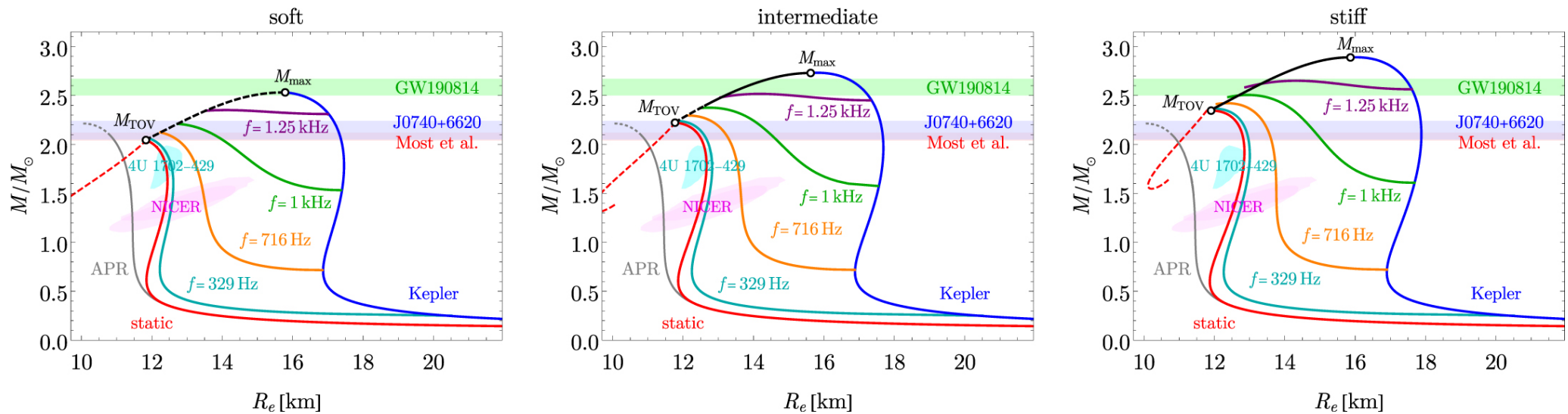
Figure 4. from Rapidly Spinning Compact Stars with Deconfinement Phase Transition null 2021 APJL 907 L37 doi:10.3847/2041-8213/abd853 https://dx.doi.org/10.3847/2041-8213/abd853 © 2021. The American Astronomical Society. All rights reserved.
