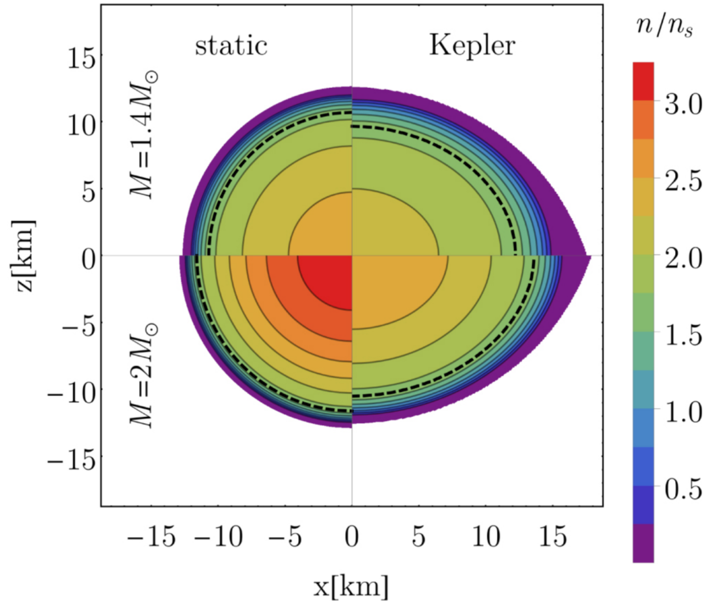
Figure 3. from Rapidly Spinning Compact Stars with Deconfinement Phase Transition null 2021 APJL 907 L37 doi:10.3847/2041-8213/abd853 https://dx.doi.org/10.3847/2041-8213/abd853 © 2021. The American Astronomical Society. All rights reserved.
