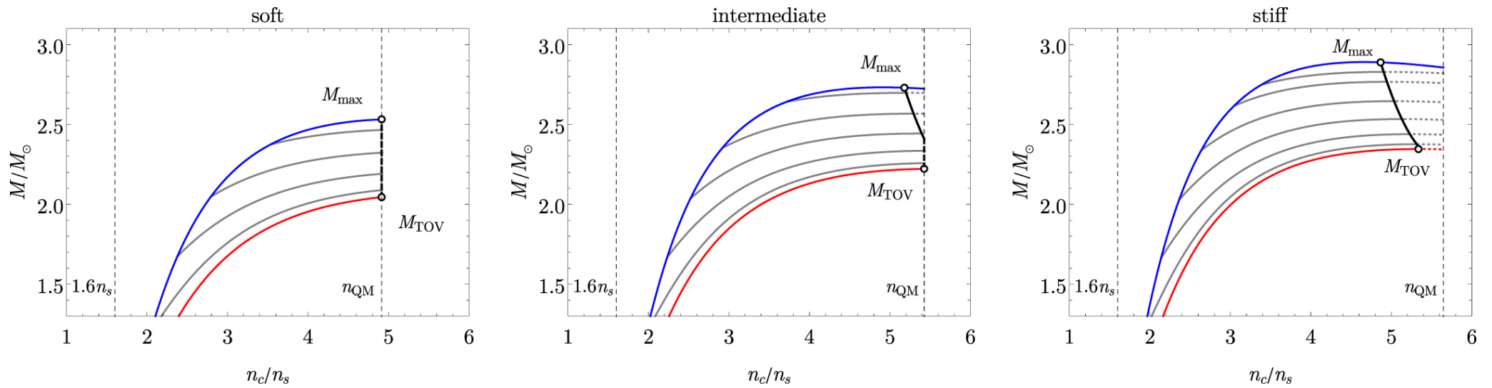
Figure 2. from Rapidly Spinning Compact Stars with Deconfinement Phase Transition null 2021 APJL 907 L37 doi:10.3847/2041-8213/abd853 https://dx.doi.org/10.3847/2041-8213/abd853 © 2021. The American Astronomical Society. All rights reserved.
