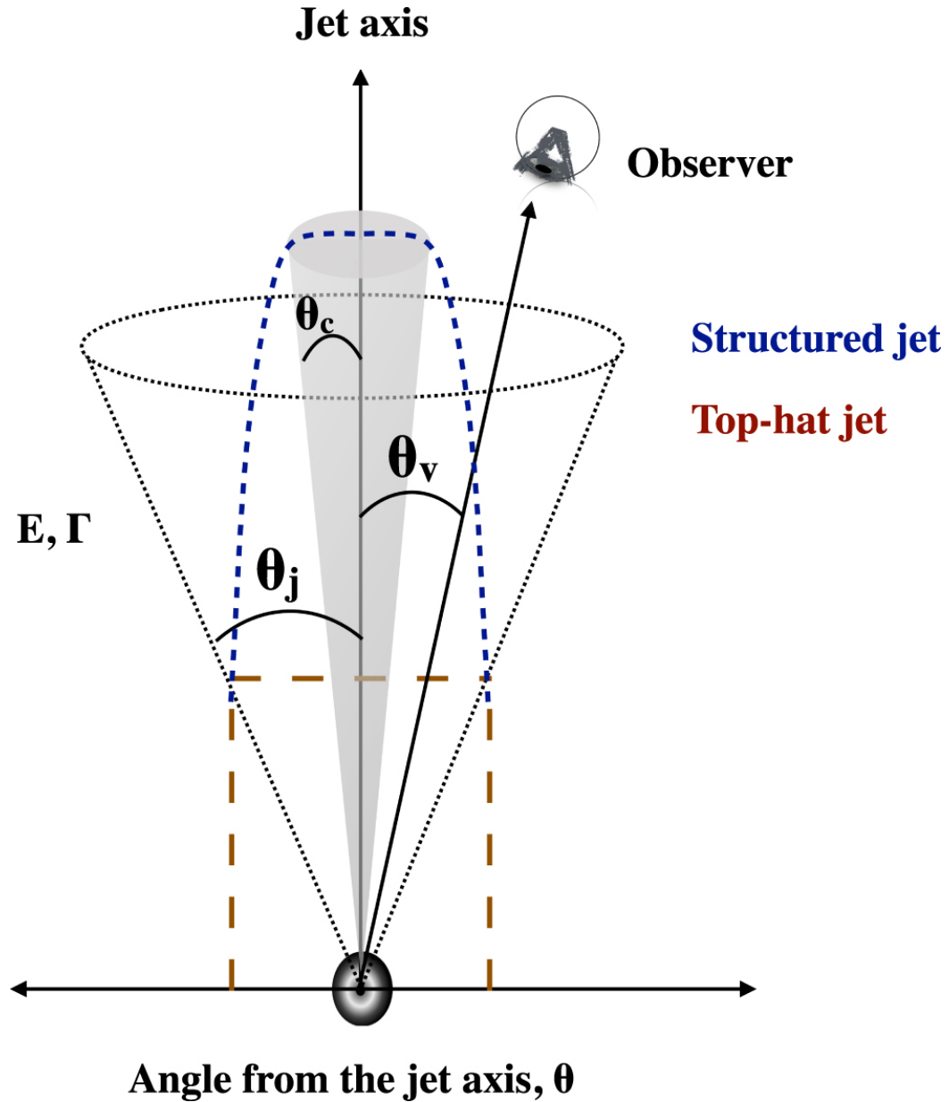
Figure 7. from Identifying Black Hole Central Engines in Gamma-Ray Bursts null 2021 APJL 908 L2 doi:10.3847/2041-8213/abd53f https://dx.doi.org/10.3847/2041-8213/abd53f © 2021. The American Astronomical Society. All rights reserved.
