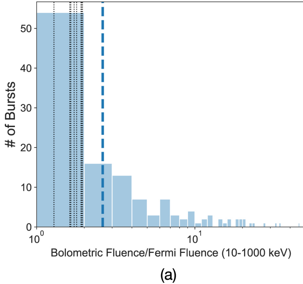
Figure 6. from Identifying Black Hole Central Engines in Gamma-Ray Bursts null 2021 APJL 908 L2 doi:10.3847/2041-8213/abd53f https://dx.doi.org/10.3847/2041-8213/abd53f © 2021. The American Astronomical Society. All rights reserved.
