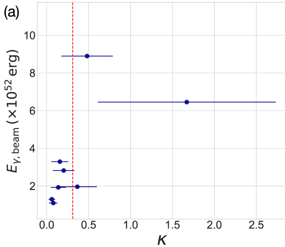
Figure 4. from Identifying Black Hole Central Engines in Gamma-Ray Bursts null 2021 APJL 908 L2 doi:10.3847/2041-8213/abd53f https://dx.doi.org/10.3847/2041-8213/abd53f © 2021. The American Astronomical Society. All rights reserved.
