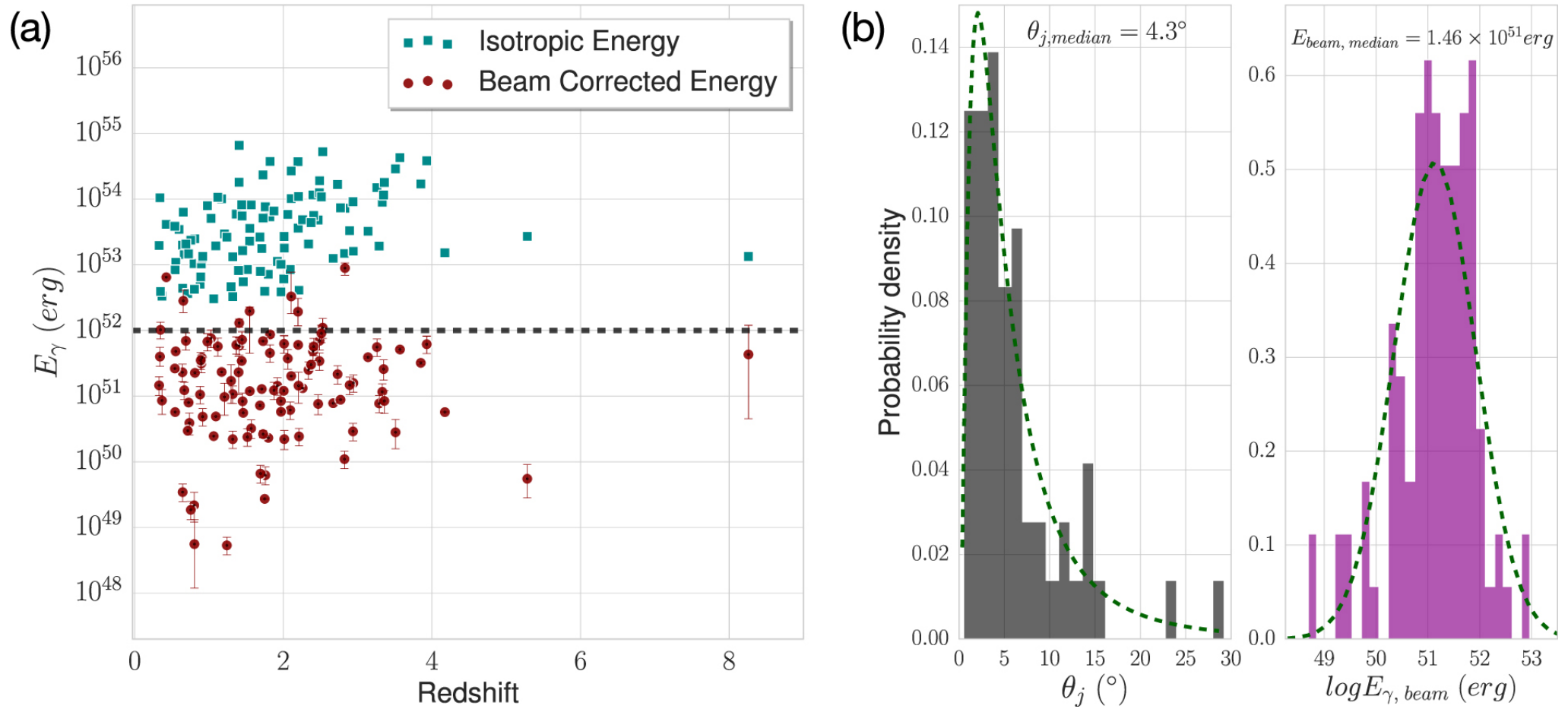
Figure 2. from Identifying Black Hole Central Engines in Gamma-Ray Bursts null 2021 APJL 908 L2 doi:10.3847/2041-8213/abd53f https://dx.doi.org/10.3847/2041-8213/abd53f © 2021. The American Astronomical Society. All rights reserved.
