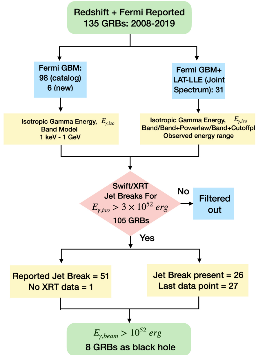
Figure 1. from Identifying Black Hole Central Engines in Gamma-Ray Bursts null 2021 APJL 908 L2 doi:10.3847/2041-8213/abd53f https://dx.doi.org/10.3847/2041-8213/abd53f © 2021. The American Astronomical Society. All rights reserved.
